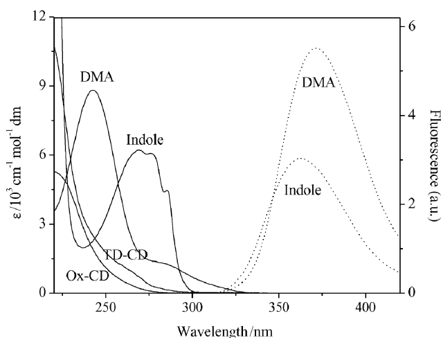
Fig. 2 UV absorption spectra of relative compounds (solid), and fluorescence emission spectra (dots) of indole and DMA upon excitation at 295 nm, in aqueous solutions.
