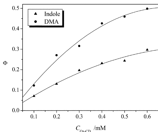
Fig. 4 Dependence of the quantum yield of splitting on concentration of Ox-CD aqueous solution containing 0.05 mM indole ( \lambda_{\text{ir}} = 295 nm) or DMA ( \lambda_{\text{ir}} = 310 nm).
