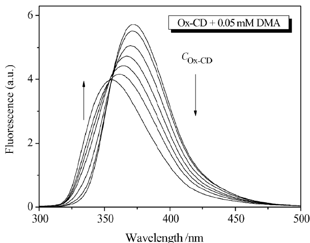
Fig. 3 Dependence of the fluorescence of 0.05 mM DMA on the concentration of Ox-CD ( 0\text{--}6.0 \times 10^{-4} M, \lambda_{\text{ex}} = 295 nm).
