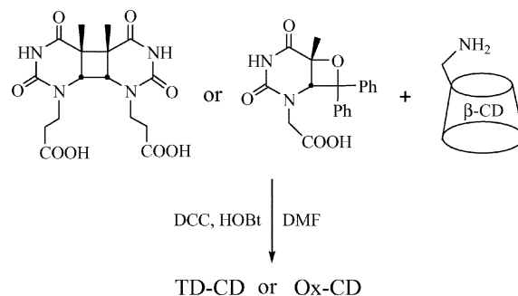
Scheme 1 Synthesis of the model compounds. Reagents and conditions: DCC, HOBt, DMF, rt, 48 h.
