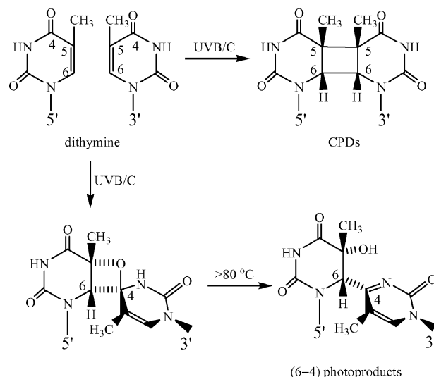
Fig. 1 Formation of the two major photoproducts between adjacent thymines in DNA under UV light, CPDs and (6–4) photoproducts.
